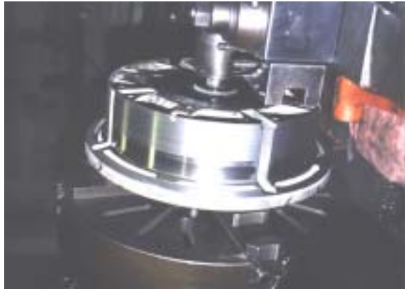
26" diameter block, carbide coated and finished to 12-16RA
