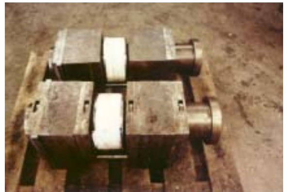
Flattening mill assemblies carbide inserts ground and polished to 6-8Ra
