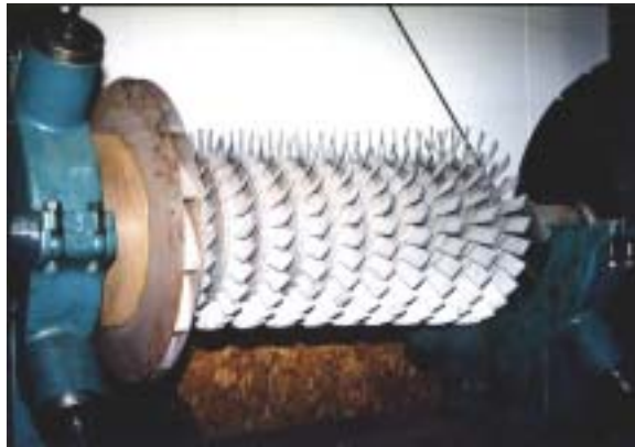
Turbo blower repaired bearings and seals
